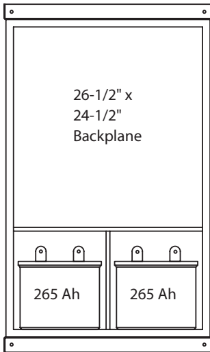
42-2 Double Wide MEGA-BOX
