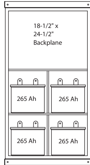
48-4 Double Wide MEGA-BOX
