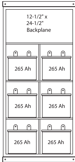
56-6 Double Wide MEGA-BOX
