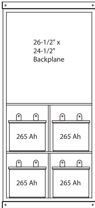
56-4 Double Wide MEGA-BOX
