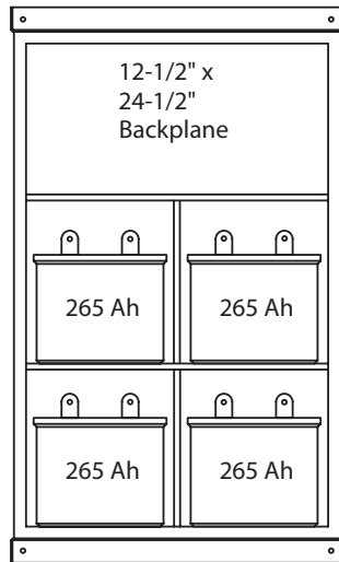
42-4 Double Wide MEGA-BOX
