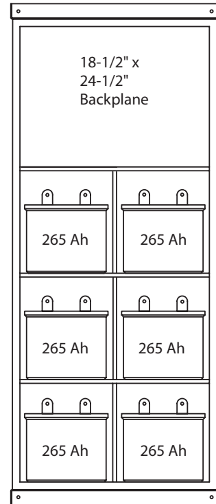
62-6 Double Wide MEGA-BOX
