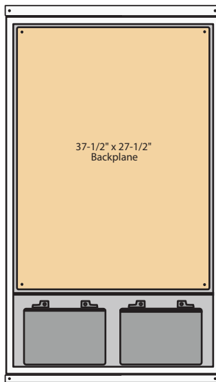
51" Double Wide TRONIX-BOX 51" x 30 1/2" x 10 1/2"
