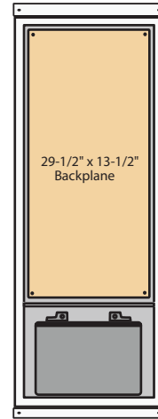
43" TRONIX-BOX 43" x 16 1/2" x 10 1/2"
