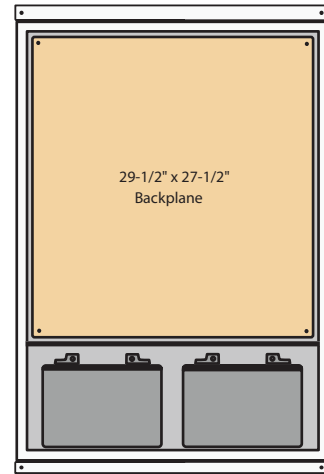
43" Double Wide TRONIX-BOX 43" x 30 1/2" x 10 1/2"
