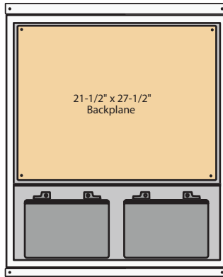
35" Double Wide TRONIX-BOX 35" x 30 1/2" x 10 1/2"
