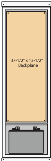
51" TRONIX-BOX 51" x 30 1/2" x 10 1/2"
