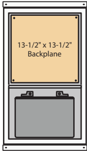
27" TRONIX-BOX 27" x 16 1/2" x 10 1/2"
