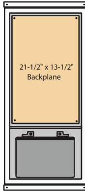
35" TRONIX-BOX 35" x 16 1/2" x 10 1/2"
