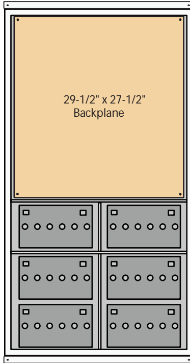
56-6 Double Wide UNI-BOX 56 x 30 1/2 x 13 1/4
