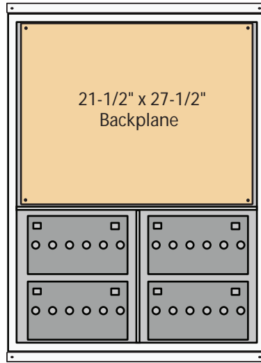
40-4 Double Wide UNI-BOX 40 x 30 1/2 x 13 1/4
