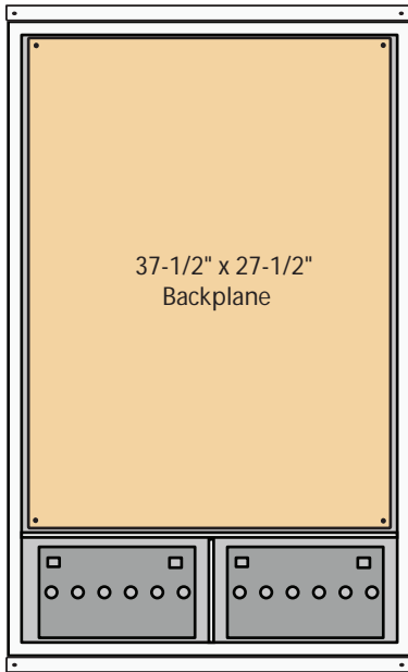
48-2 Double Wide UNI-BOX 48 x 30 1/2 x 13 1/4
