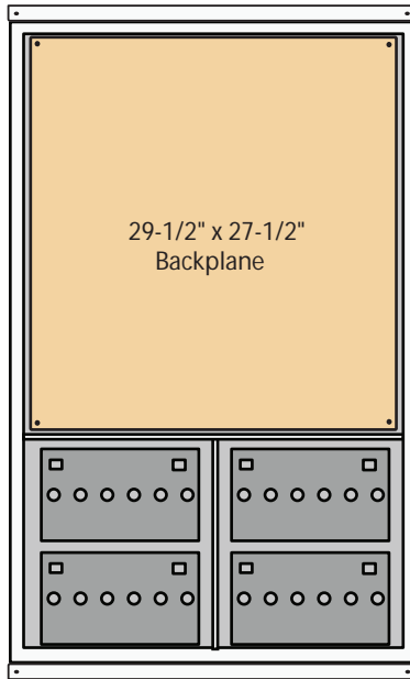
48-4 Double Wide UNI-BOX 48 x 30 1/2 x 13 1/4
