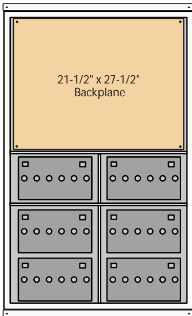
48-6 Double Wide UNI-BOX 48 x 30 1/2 x 13 1/4
