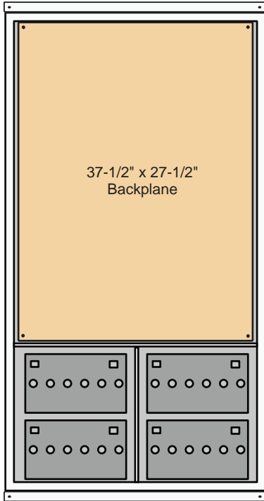
56-4 Double Wide UNI-BOX 56 x 30 1/2 x 13 1/4
