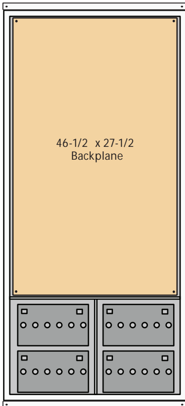
65-4 Double Wide UNI-BOX 65 x 30 1/2 x 13 1/4
