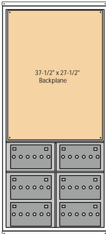
65-6 Double Wide UNI-BOX 65 x 30 1/2 x 13 1/4
