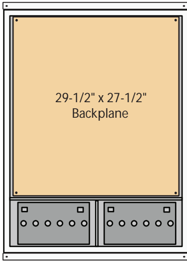
40-2 Double Wide UNI-BOX 40 x 30 1/2 x 13 1/4
