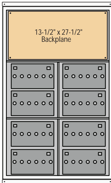
48-8 Double Wide UNI-BOX 48 x 30 1/2 x 13 1/4
