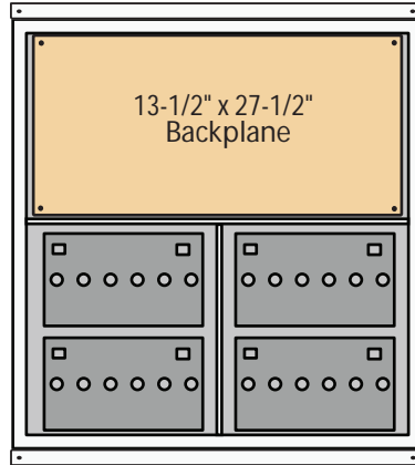
32-4 Double Wide UNI-BOX 32 x 30 1/2 x 13 1/4
