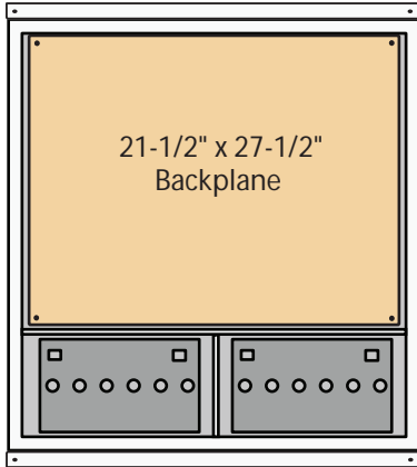
32-2 Double Wide UNI-BOX 32 x 30 1/2 x 13 1/4
