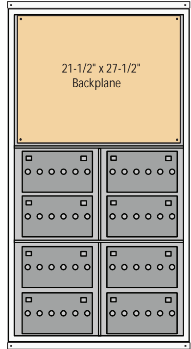
56-8 Double Wide UNI-BOX 56 x 30 1/2 x 13 1/4
